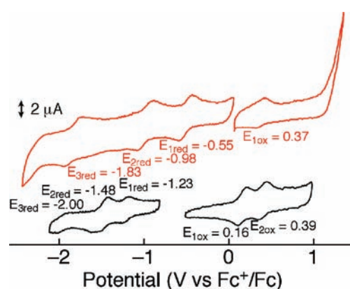
Figure 4. Cyclic voltammetry data for 3a (bottom, black lines) and 4a (top, red lines). Cyclic voltammograms were acquired from 1.0 mM solutions of analyte in 0.1 M n\text{Bu}_4\text{NClO}_4/o\text{-DCB} . Ferrocene was used as an internal standard and set to 0 V.
